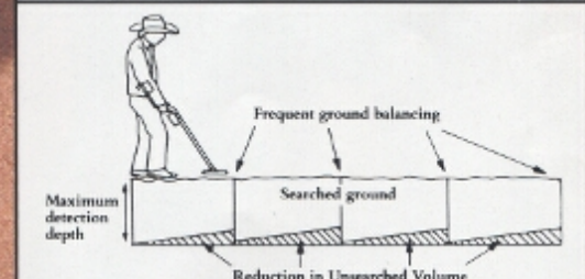
To compensate for loss of detection effect with a conventional detector, a hard-working goldseeker will ground balance frequently - a time-consuming, not entirely effective method.
