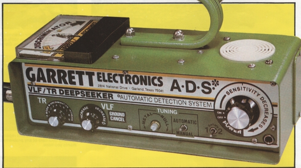
GARRETT'S MASTER HUNTER A-D-S DEEPSEEKER
